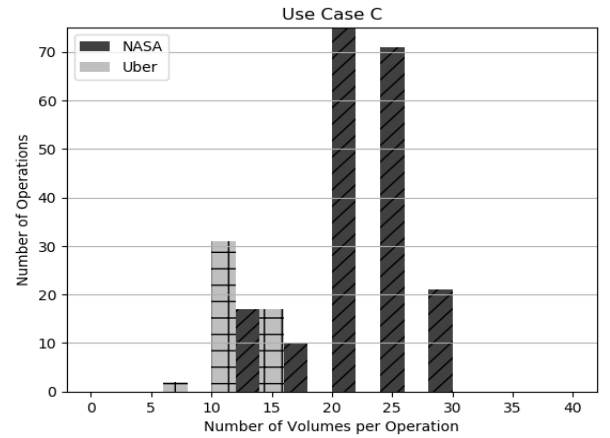
Fig. 11. Number of volumes per operation, Use Case C, Baseline Condition for NASA and Uber flights.
