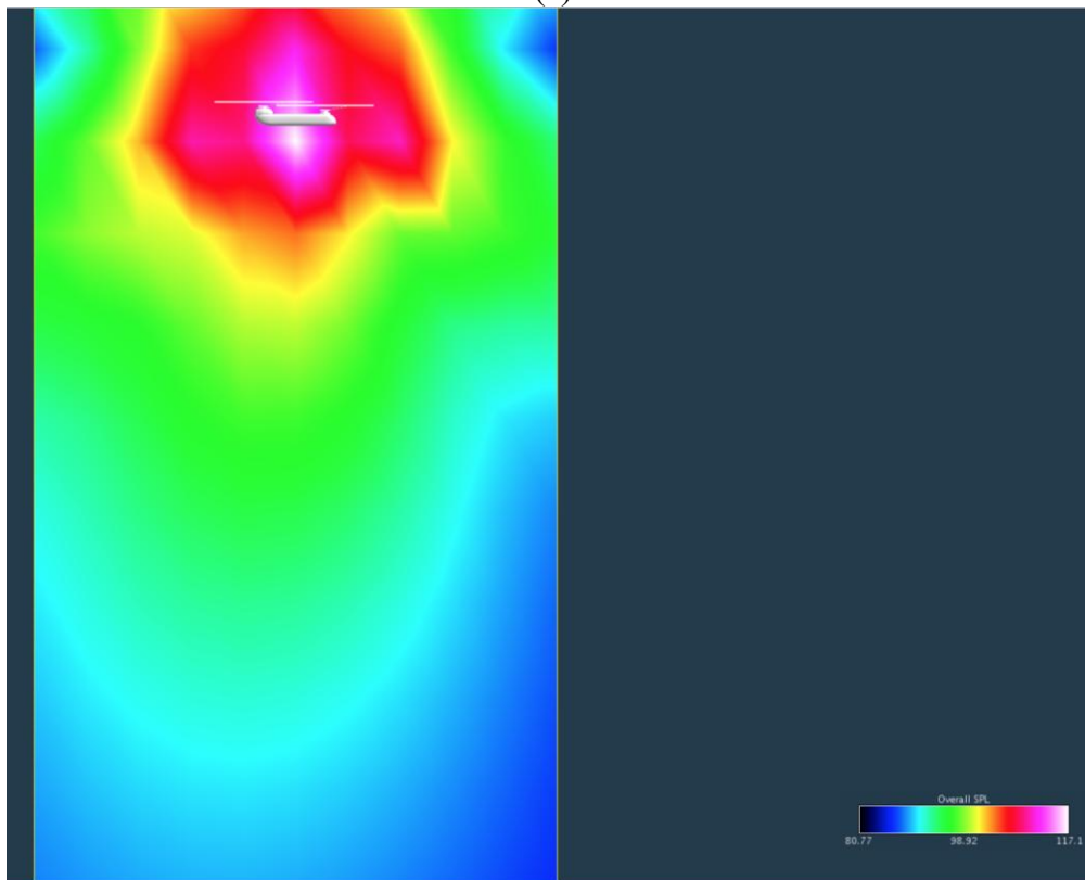
Figure B7. RotCFD OASPL prediction for 30-PAX electric tandem helicopter reference design for 150m AGL static (HOGE) operation: (a) orthogonal view and (b) side view.
