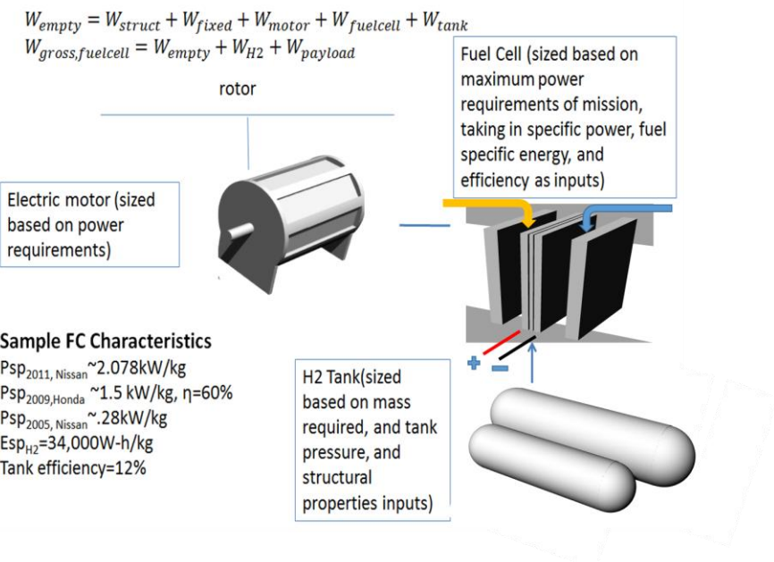
Figure F4. Fuel-cell power system.
