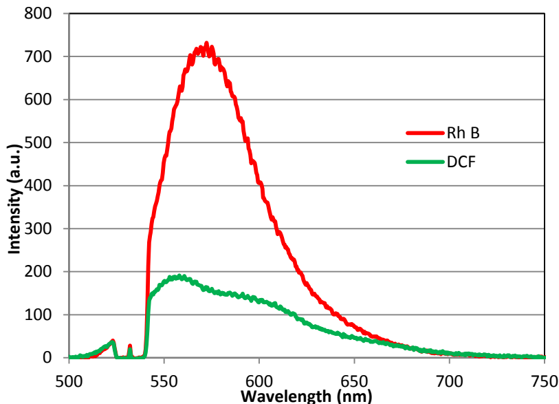
Figure 6. Comparison of fluorescence of Rhodamine B and DCF dye-doped PSLs, both excited at 532 nm
