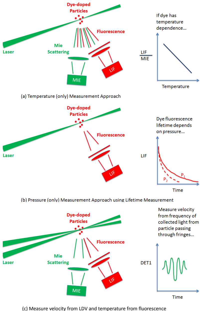
Figure 1. Three potential measurement schemes using dye-doped polystyrene latex spheres.
